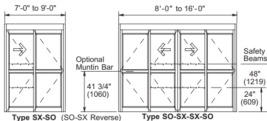
Type SX-SO (SO-SX Reverse)
