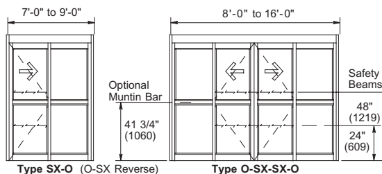
Type SX-O (O-SX Reverse)
